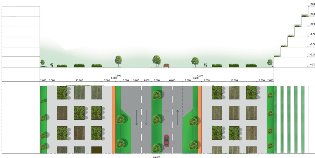
Detailed Plan and Section for the main street.
